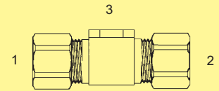
BC-2602 - Tee (1) (2) Male Compression (3) Fem. Pipe
