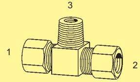
BC-2601 - Tee (1) (2) Compression (3) Male Pipe
