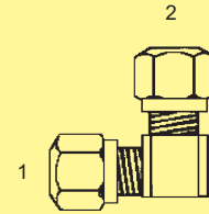
BAB-N-2500 - 90° (1) (2) Air Brake
