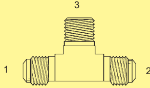
BF-2601 - Tee (1) (2) Male 45° (3) Male Pipe
