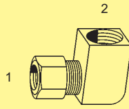
BC-2502 - 90° (1) Compression (2) Fem. Pipe
