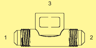
BF-2602-F - Tee (Forged) (1) (2) Male 45° (3) Fem. Pipe
