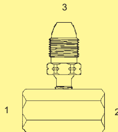
B-POL-2001-CV - Tee Manifold Block Tee Assembly with Check Valve (1) (2) Fem. POL (3) Male POL B-POL-2001-CV
