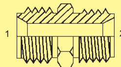
BP-BS-5176 - Str. (1) (2) Male Ball Seat
