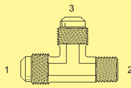
BF-2605-F - Tee (Forged) (1) (3) Male 45° (2) Male Pipe
