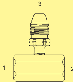
B-POL-2001 - Tee Manifold Block Tee Assembly (1) (2) Fem. POL (3) Male POL B-POL-2001
