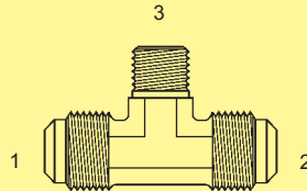
BF-2601-F - Tee (Forged) (1) (2) Male 45° (3) Male Pipe
