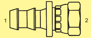
BPO-2280 - Str. (1) Hose Barb (2) Fem. Pipe Swivel Gasket Seat
