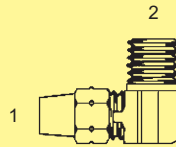
BC-L-2501 - 90° (1) Compression (2) Male Pipe
