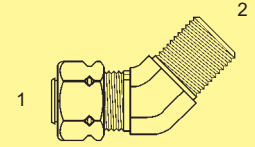
BC-SA-2503 - 45° (1) Compression (2) Male Pipe
