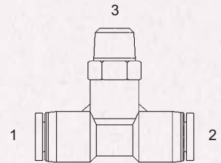
CPC-SB-2601-S - Tee (1) (2) Tube (3) Male Pipe Swivel
