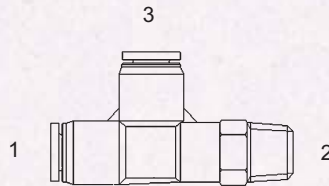
CPC-2605-S - Tee (1) (3) Tube (2) Male Pipe Swivel
