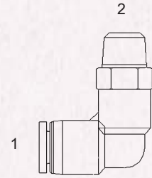
CPC-SB-2501-S - 90° (1) Tube (2) Male Pipe Swivel
