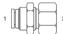
CPC-2705-LN - Str. (1) Bulkhead Tube (2) Fem. Pipe CPC-2705-LN-03-02 CPC-2705-LN-03-04 CPC-2705-LN-04-02 CPC-2705-LN-04-04 CPC-2705-LN-05-02 CPC-2705-LN-05-04 CPC-2705-LN-05-06 CPC-2705-LN-06-04 CPC-2705-LN-06-06 CPC-2705-LN-08-06 CPC-2705-LN-08-08 CPC-2705-LN-5/32-02 CPC-2705-LN-5/32-04
