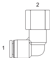
CPC-2502-S - 90° (1) Tube (2) Fem. Pipe Swivel
