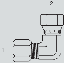
Y-FL-6500 - 90° (1) Male Flareless (2) Fem. Flareless Swivel
