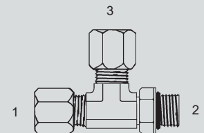
Y-FL-6804-NWO - Tee (1) (3) Male Flareless (2) Adj. O-Ring
