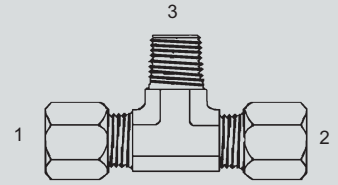
Y-FL-2601 - Tee (1) (2) Male Flareless (3) Male Pipe
