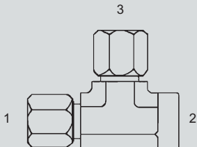
Y-FL-2606 - Tee (1) (3) Male Flareless (2) Fem. Pipe
