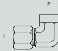
Y-FL-2502 - 90° (1) Male Flareless (2) Fem. Pipe
