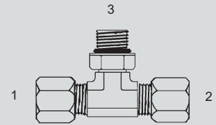
Y-FL-6803-NWO - Tee (1) (2) Male Flareless (3) Adj. O-Ring
