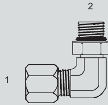
Y-FL-6801-NWO - 90° (1) Male Flareless (2) Adj. O-Ring
