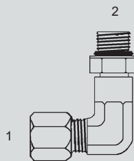
Y-FL-6801-L-NWO - 90° (1) Male Flareless (2) Adj. O-Ring-Long
