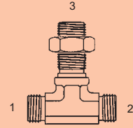
Y-OFS-2703-F-LN - Tee (1) (2) Male OFS (3) OFS Bulkhead with Locknut
