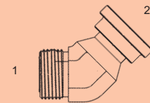
Y-OFS-1703-F-62 - 45° (1) Male OFS (2) O-Ring Flange Code 62
