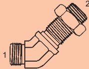
Y-OFS-2702-F-LN - 45° (1) Male OFS (2) OFS Bulkhead with Locknut
