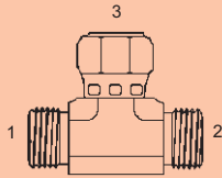
Y-OFS-6600-F - Tee (1) (2) Male OFS (3) Fem. OFS Swivel
