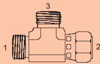
Y-OFS-6602-F - Tee (1) (3) Male OFS (2) Fem. OFS Swivel
