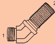
Y-OFS-2702-F - 45° (1) Male OFS (2) OFS Bulkhead
