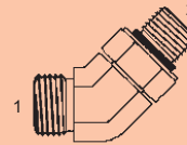
Y-OFS-6802-F-NWO - 45° (1) Male OFS (2) Adj. O-Ring
