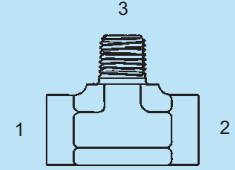
Y-SS-5604 - Tee (1) (2) Fem. Pipe (3) Male Pipe
