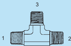
Y-SS-5600 - Tee (1) (2) (3) Male Pipe
