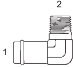
Y-4501-F - 90° (1) Beaded (2) Male Pipe
