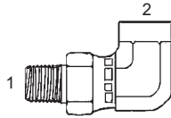
Y-5502-F-S - 90° (1) Male Pipe Swivel (2) Fem. Pipe
