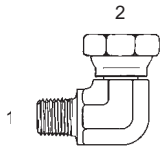
RESTRICTOR Y-1501-F-R - 90° (1) Male Pipe (2) Fem. Pipe Swivel
