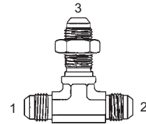
Y-2703-F-LN - Tee (1) (2) Male 37° (3) Bulkhead 37° w/ Locknut
