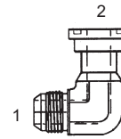
Y-1704-F-61 - 90° (1) Male 37° (2) O-Ring Flange Code 61
