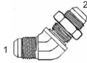
Y-2702-F-LN - 45° (1) Male 37° (2) Bulkhead 37° w/ Locknut
