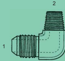
BST-MJ-2501 - 90°
