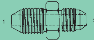
JISM-MJ-2403 - Str. (1) Male 30° Metric Komatsu (2) Male 37°
