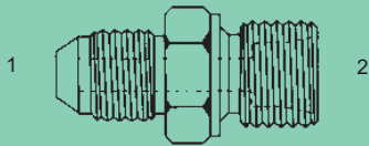
MFL-MJ-3901 - Str. (1) Male 37° (2) Male Metric Dual Purpose (Port of Tube) Light
