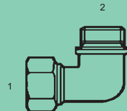
MFL-MT-2501 - 90°
