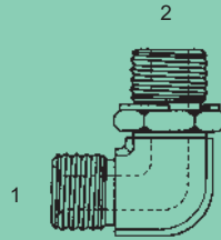
BPP-7801-NW0 - 90° (1) Male BPP (2) Male BPP Adj. O-Ring
