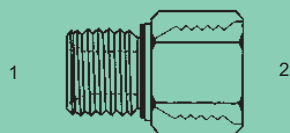
M-FB-6410-WO - Str. (1) Male Metric w/ Washer O-Ring (2) Fem. O-Ring (SAE)
