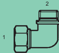
MFL-M-2501-H - 90° (1) Male Flareless (2) Male Metric Parallel w/ Cutting Face Seal Heavy
