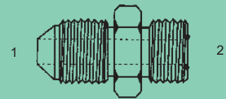
JISM-OFS-2403 - Str. (1) Male 30° Metric Komatsu (2) Male O-Ring Face Seal (SAE)
