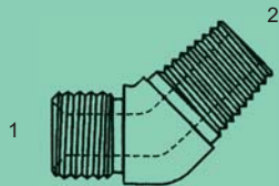
BPP-BST-5501 - 45° (1) Male BPP (2) Male BSPT
