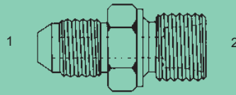
MFL-MJ-3901-H - Str. (1) Male 37° (2) Male Metric Dual Purpose (Port or Tube) Heavy
