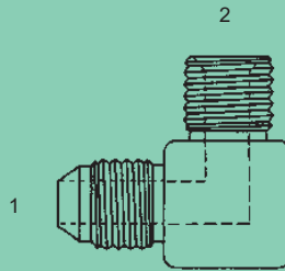
BPP-MJ-2501 - 90°
