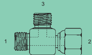
BPP-1662 - Tee (1) (3) Male BPP (2) Fem. BPP Swivel
