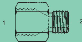
JISBP-MOFS-2406 - Str. (1) Fem. 30° BPP (Flare) (2) Male O-Ring Face Seal (SAE)
