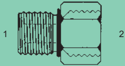
BPP-6410-EO - Str. (1) Male BPP w/ Peflex Seal (2) Fem. BPP
