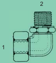
MFL-BPP-6801-H-NWO - 90°
