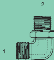
BPP-OFS-6801-NWO - Str. (1) Male O-Ring Face Seal (SAE) (2) Male BPP Adj. O-Ring w/ Retainer Washer
