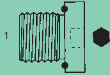
BPP-6408-HHP-EO - Str. (1) Male BPP Hollow Hex Plug w/ Peflex Seal
