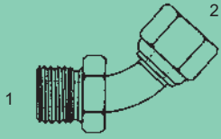
BPP-1503-L - 45° (1) Male BPP (2) Fem. BPP Swivel - Long
