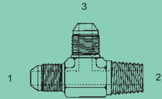
BST-MJ-2605 - Tee
