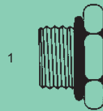
M-6408-ISO - Str. (1) Metric Hex Plug (Parallel) w/ ISO O-Ring
