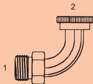
OFS-1704-61 - 90° Forged (1) Male OFS (2) O-Ring Flange Code 61
