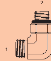
OFS-6801-NWO - 90° (1) Male OFS (2) Adj. O-Ring
