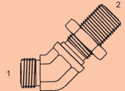
OFS-2702-LN - 45° (1) Male OFS (2) OFS Bulkhead with Locknut
