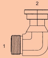
OFS-1704-F-61 - 90° Forged (1) Male OFS (2) O-Ring Flange Code 61
