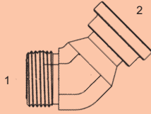
OFS-1703-F-62 - 45° Forged (1) Male OFS (2) O-Ring Flange Code 62
