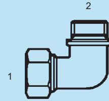
SS-MFL-BST-2501 - 90° (1) Male Flareless (2) Male BSPT Light
