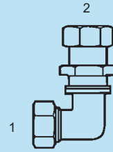
SS-MFL-2701-H-LN - 90° (1) Male Flareless (2) Male Flareless Bulkhead w/ Lock Nut Heavy
