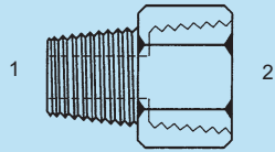
SS-BST-FP-5405 - Str. (1) Male BSPT (2) Fem. NPT Pipe
