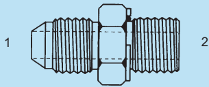
SS-BPP-MJ-6400-WO - Str. (1) Male 37° (2) Male BPP w/ Washer O-Ring
