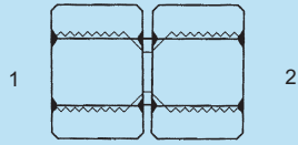
SS-MFL-6565 - Str. (1) (2) Fem. Flareless Swivel Light
