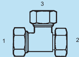
SS-MFL-6602 - Tee (1) (3) Male Flareless (2) Fem. Flareless Swivel Light
