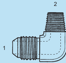
SS-BST-MJ-2501 - 90° (1) Male 37° (2) Male BSPT
