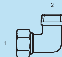
SS-MFL-MP-2501 - 90° (1) Male Flareless (2) Male NPT Light
