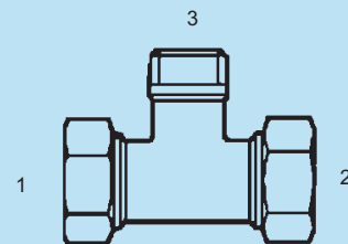
SS-MFL-MP-2601 - Tee (1) (2) Male Flareless (3) Male NPT Light
