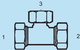
SS-MFL-6600 - Tee (1) (2) Male Flareless (3) Fem. Flareless Swivel Light
