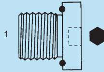
SS-BPP-6408-HHP-EO - Str. (1) Male BPP Hollow Hex Plug w/ Peflex Seal
