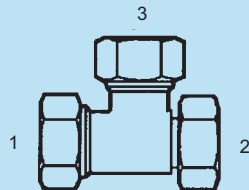
SS-MFL-6602-H - Tee (1) (3) Male Flareless (2) Fem. Flareless Swivel Heavy
