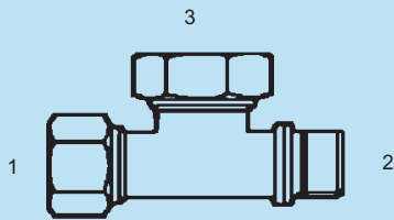
SS-MFL-BST-2605 - Tee (1) (3) Male Flareless (2) Male BSPT Light
