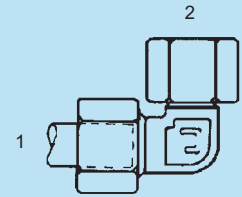
SS-MFL-6500 - 90° (1) Male Flareless (2) Fem. Flareless Swivel Light
