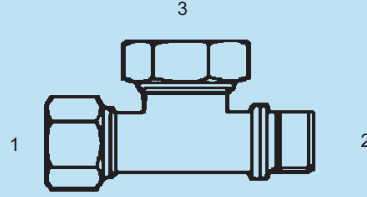
SS-MFL-BST-2605-H - Tee (1) (3) Male Flareless (2) Male BSPT Heavy
