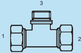
SS-MFL-BST-2601-H - Tee (1) (2) Male Flareless (3) Male BSPT Heavy
