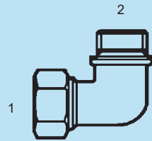
SS-MFL-BST-2501-H - 90° (1) Male Flareless (2) Male BSPT Heavy
