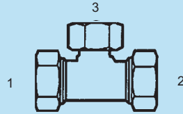
SS-MFL-6600-H - Tee (1) (2) Male Flareless (3) Fem. Flareless Swivel Heavy
