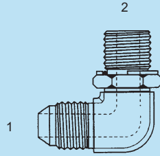
SS-BPP-MJ-6801-NWO - 90° (1) Male 37° (2) Male BPP Adj. O-Ring w/ Retainer Washer
