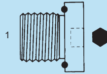
SS-BPP-6408-HHP-EO - Str. (1) Male BPP Hollow Hex Plug w/ Peflex Seal
