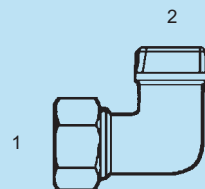
SS-MFL-MP-2501 - 90° (1) Male Flareless (2) Male NPT Light
