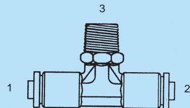
SSPC-2601-S - Tee (1) (2) Tube (3) Male Pipe Swivel
