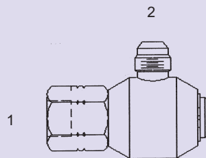
SLS-OFS-2510 - 90° (1) Fem. O-Ring Face Seal - Stem (2) Male JIC - Barrel
