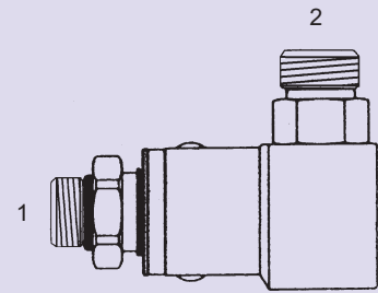
SLS-OFS-6846-5K-O - 90° 5000 PSI (1) Male O-Ring - Stem (2) Male O-Ring Face Seal - Barrel
