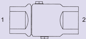
SLS-5000-HP - Str. High Pressure - 10,000 PSI (1) Fem. Pipe - Stem (2) Fem. Pipe - Barrel
