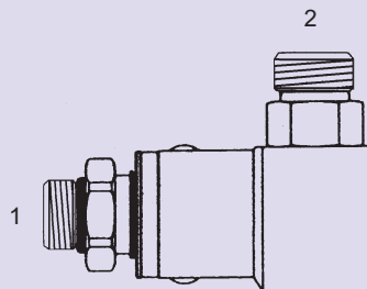
SLS-OFS-6846-4K-O - 90° 4000 PSI (1) Male O-Ring - Stem (2) Male O-Ring Face Seal - Barrel
