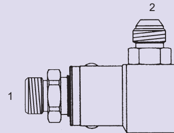
SLS-OFS-6861 - 90° (1) Male O-Ring Face Seal - Stem (2) Male JIC - Barrel
