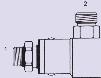
SLS-OFS-6846-LH - 90° 5000 PSI Large Hex (1) Male O-Ring - Stem (2) Male O-Ring Face Seal - Barrel
