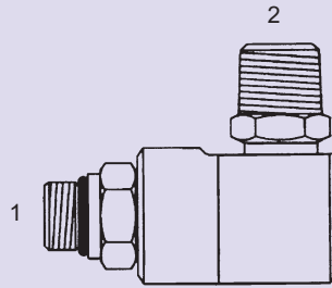
SLS-6806-O - 90° (1) Male O-Ring - Stem (2) Male Pipe - Barrel
