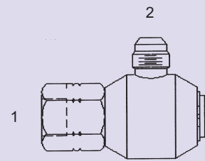
SLS-OFS-2510-5K - 90° 5000 PSI (1) Fem. O-Ring Face Seal - Stem (2) Male JIC - Barrel
