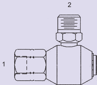
SLS-OFS-2507 - 90° (1) Fem. O-Ring Face Seal - Stem (2) Male Pipe - Barrel
