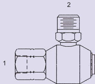
SLS-OFS-2509 - 90° (1) Fem. Pipe Swivel - Stem (2) Fem. O-Ring Face Seal - Barrel
