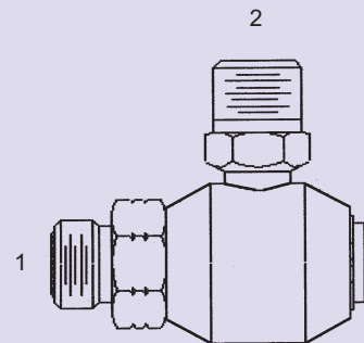
SLS-OFS-2567 - 90° (1) Male O-Ring Face Seal - Stem (2) Male Pipe - Barrel
