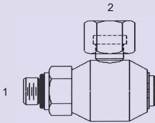
SLS-OFS-6840-5K-O - 90° 5000 PSI (1) Male O-Ring - Stem (2) Fem. O-Ring Face Seal Swivel - Barrel
