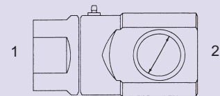
SLS-5504-SB - 90° (1) Fem. Pipe - Stem (2) Fem. Pipe - Barrel (Short Body)
