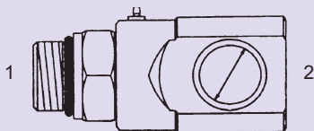
SLS-6805-SB-O - 90° (1) Male O-Ring - Stem (2) Fem. Pipe - Barrel (Short Body)
