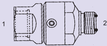
SLS-OFS-2406 - Str. (1) Fem. O-Ring Face Seal - Stem (2) Male O-Ring Face Seal - Barrel
