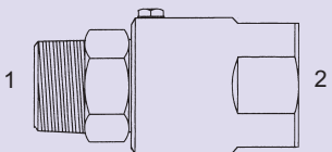
SLS-5405 - Str. (1) Male Pipe - Stem (2) Fem. Pipe - Barrel
