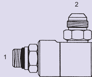
SLS-6841-O - 90° (1) Male O-Ring - Stem (2) Male JIC - Barrel
